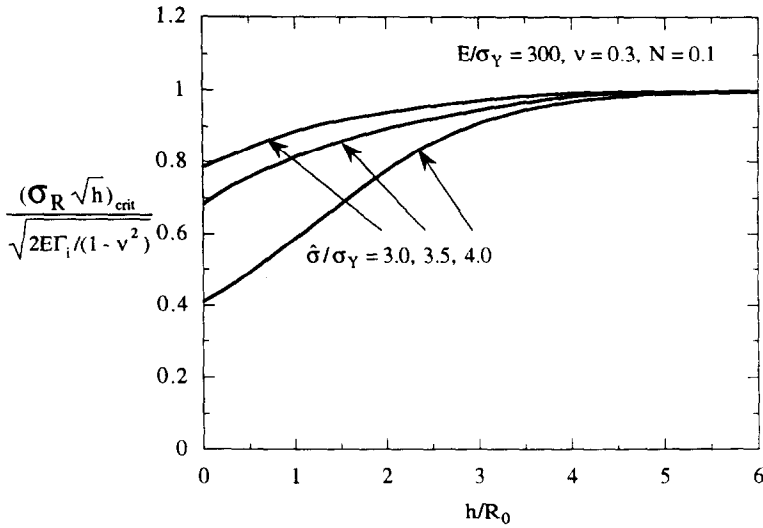
Fig. 4. Critical combination of \sigma\sqrt{h} as a function of film thickness for yielding in the substrate according to the EPZ model. For h/R_0 > 5 , the critical combination for delamination becomes independent of film thickness. The interface toughness \Gamma_i applies for “thick” films in this range. For \sigma_R > 0 .
