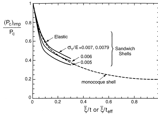
Fig. 8. Influence of face sheet yield stress on the relation between the buckling load and the imperfection amplitude. The amplitude for the imperfection for the elastic monocoque shell is normalized by the shell thickness, while the effective thickness is used for the sandwich shells. Plastic yielding of the face sheets has essentially no effect for yield stresses above \sigma_Y/E = 0.007 . The shell parameters are given in Eq. (5.1). The core is elastic.
