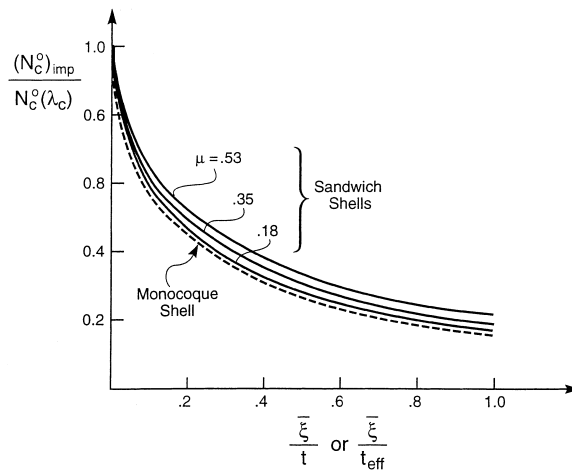
Fig. 3. Ratio of the elastic buckling load of the imperfect shell to that of the perfect shell as a function of the amplitude of the axisymmetric imperfection, \bar{\xi} . For Koiter (1963) the result for the monocoque shell, the imperfection amplitude is normalized by the shell thickness, t . For the results of Tennyson and Chan (1990) for sandwich shells, the imperfection amplitude is normalized by the effective thickness, t_{\text{eff}} , defined by Eq. (4.3).
