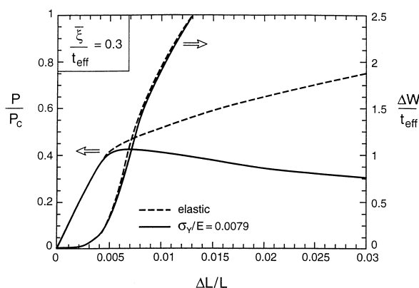
Fig. 7. Load versus end shortening for both an elastic face sheets and face sheets with yield stress equal to the stress in the sheets at the buckling load of the perfect shell. Also shown is the development of the amplitude of the non-axisymmetric deflection, \Delta w . The definition of the buckling load of the imperfect shells used here is that load associated with attainment of \Delta w/t_{\text{eff}} = 1/2 . The shell parameters are given in Eq. (5.1) and \bar{\xi}/t_{\text{eff}} = 0.3 . The core is elastic.
