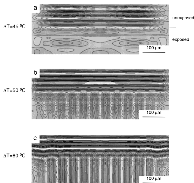
Figure 5. Simulated buckling patterns on infinitely long, parallel strips as the temperature of the system is decreased. The top half of each pattern was not exposed to UV light, and the bottom half was exposed to UV light. (a) Start of buckling on a nonexposed area ( \Delta T = 45^\circ\text{C} ). The buckles are the long parallel lines parallel to the interface of the exposed and unexposed regions. (b) Start of buckling on UV-exposed area ( \Delta T = 50^\circ\text{C} ). The buckles in the unexposed region are perpendicular to the interface of the exposed and unexposed regions. (c) Wrinkling of longitudinal buckles ( \Delta T = 80^\circ\text{C} ). The contours show the heights of the surface.
