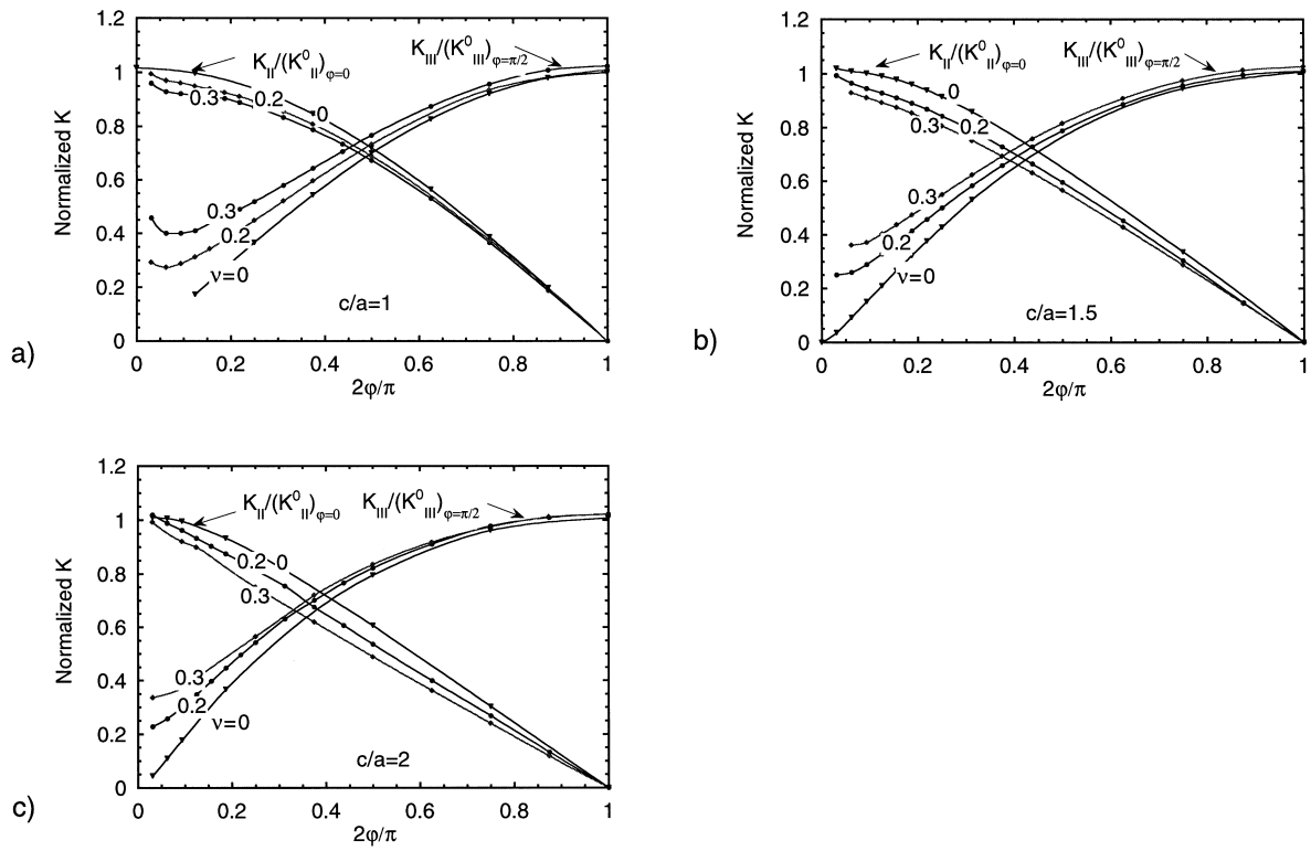
Fig. 8. Normalized distributions of the stress intensity factors for the semi-elliptical surface crack subject to nonzero \sigma_{12}^0 for \nu = 0, 0.2 and 0.3 : (a) c/a = 1 , (b) c/a = 1.5 and (c) c/a = 2 .
