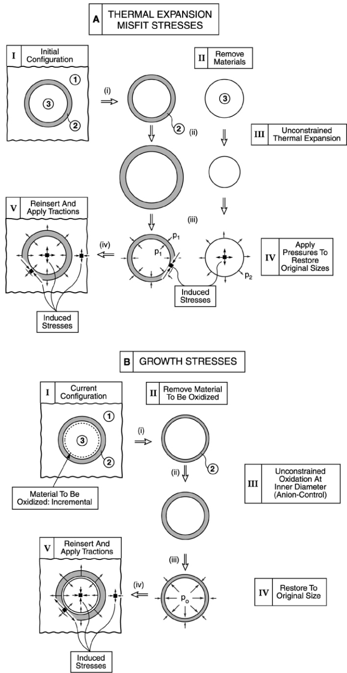
Fig. B1. The stresses that develop around spherical imperfections illustrated by using the “Eshelby” procedure. (A) Thermal expansion misfit, (B) anion-controlled TGO growth. The three regions are as follows: (1) the TBC, (2) the TGO and (3) the bond coat/substrate combinations.
