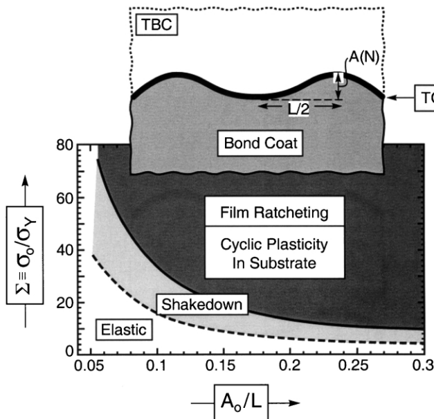
Fig. 14. Bree diagram for a TGO governing ratcheting and shakedown [37].
