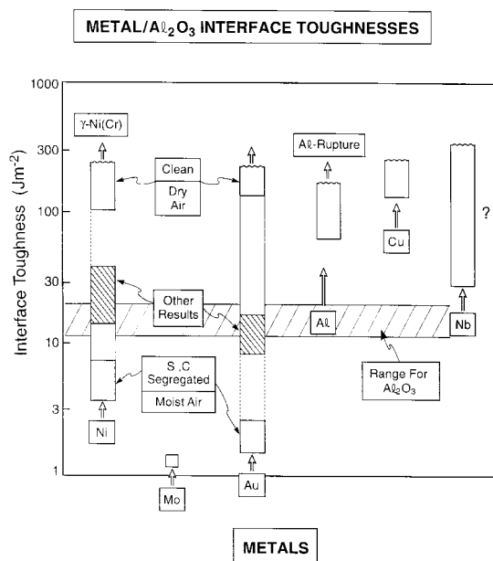
Fig. 7. The range of toughnesses found between \text{Al}_2\text{O}_3 and various metals. Note that many results reside in discrete domains that depend on “cleanliness”. Only interfaces with Mo are consistently brittle. The question mark against the Nb/ \text{Al}_2\text{O}_3 system pertains to the invalid method used to ensure the toughness (see Table 1).
