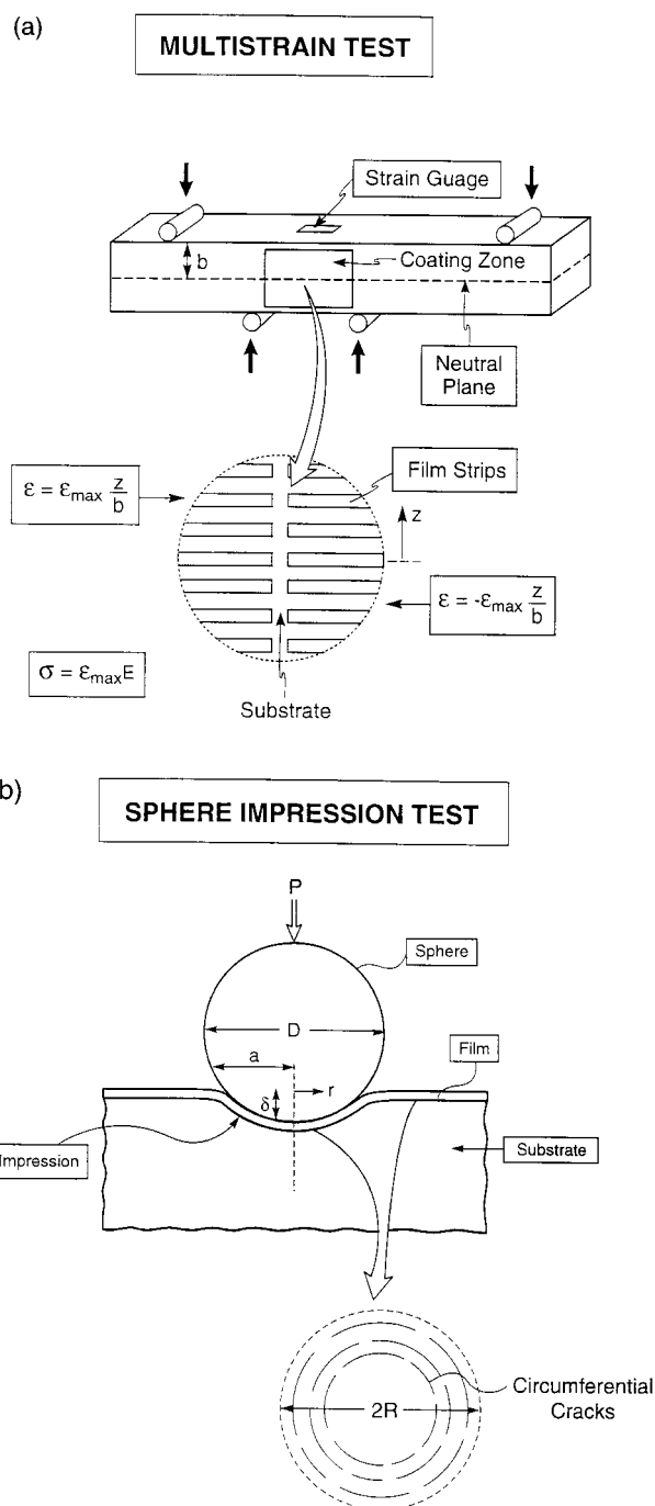
Fig. 5. Tests used to measure the toughness of interfaces between thin films and a ductile substrate: (a) multistrain test; (b) sphere impression test.
