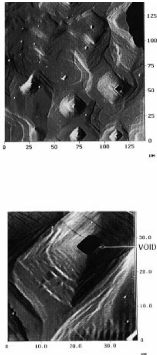
Fig. 11. AFM images of a Au fracture surface from the specimen shown in Fig. 10 revealing slip steps emanating from initial voids in the Au at the interface.
