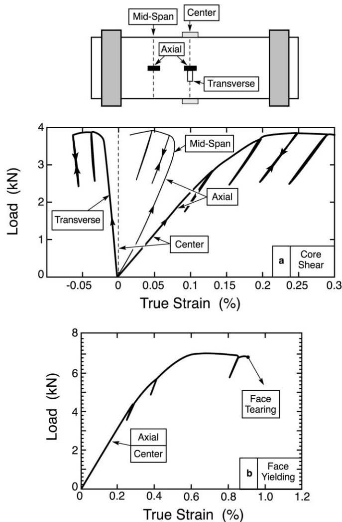
Fig. 13. The face layer strains as a function of bending load; (a) The panel having the smallest truss radius that fails by plastic buckling of the core. The mid-span gage is located on the side that experiences plastic buckling; (b) The panel with the largest truss that fails by face yielding.
