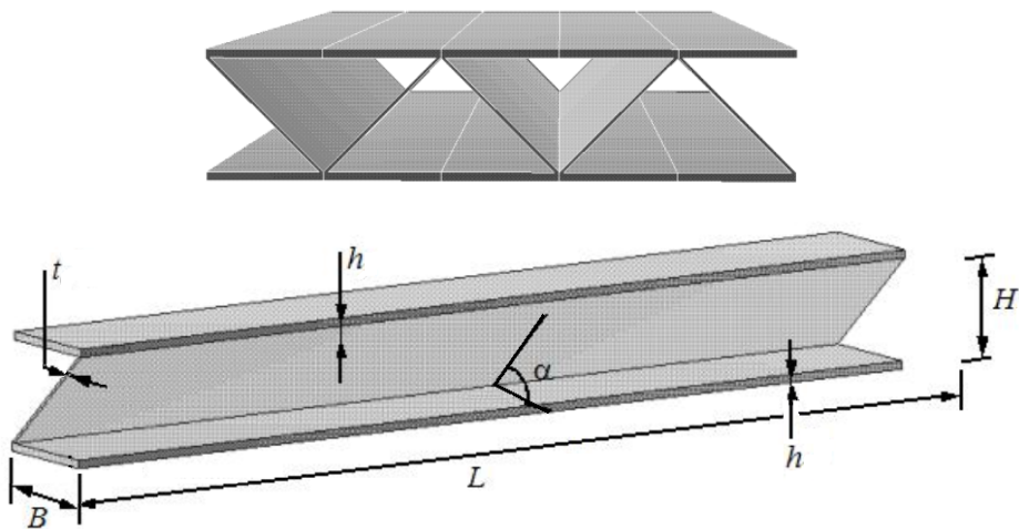
(b) folded sandwich plate
