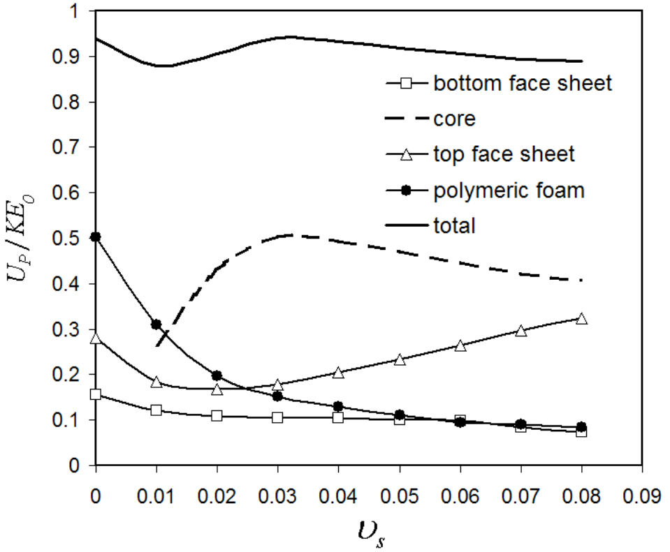
Figure 15: The plastic dissipation in foam-filled square honeycomb sandwich plates (H200 Polymeric Foam) versus the volume fraction of the core occupied by steel, v_s , at t/(L/\sqrt{\sigma_{Ys}/\rho_s}) = 1 . All sandwich plates have M/(\rho_s L) = 0.02 , H/L = 0.1 , B/H = 1 and subjected to I/(M\sqrt{\sigma_{Ys}/\rho_s}) = 0.25 .
