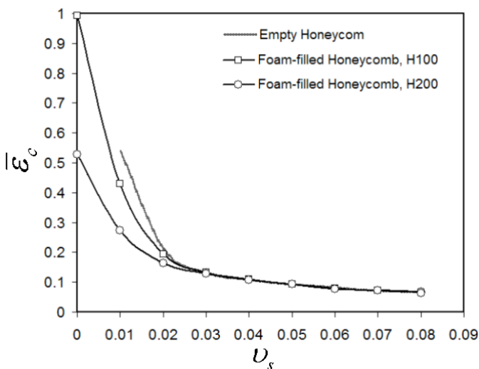
(b) The maximum nominal compressive strain in the core, \bar{\epsilon}_c , of empty and foam-filled square honeycomb sandwich plates versus the volume fraction of the core occupied by steel, U_s
