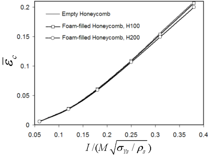
(b) The maximum nominal compressive strain in the core, \bar{\varepsilon}_c , of empty and foam-filled square honeycomb sandwich plates versus normalized momentum impulse, I/(M\sqrt{\sigma_{Ys}/\rho_s}) .
