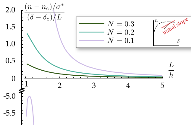
Fig. 4. The initial slope of the post-bifurcation load-elongation behavior for the block of nonlinear power-law material, as obtained by the initial post-bifurcation analysis in Eq. (3.18).
