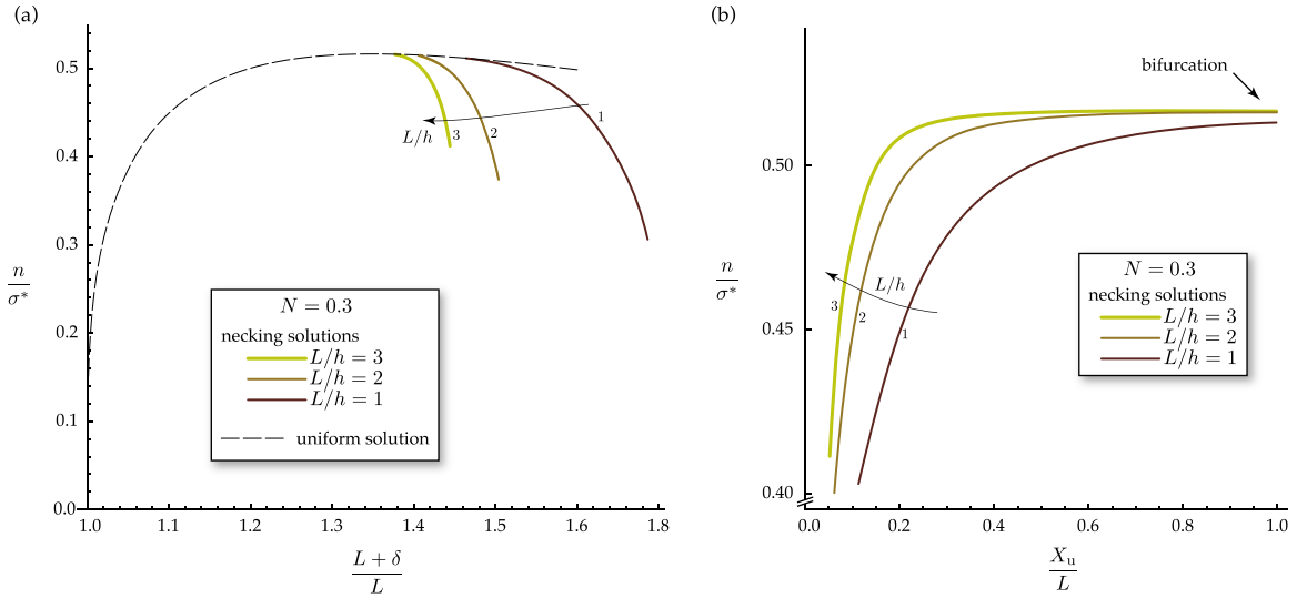
Fig. 6. (a) Load-overall stretch response and (b) load versus location of the boundary between the loading and unloading regions for three ratios of the initial half-length to thickness. The block material is elastic-plastic with N=0.3 and \sigma^*/E = 0.003 .
