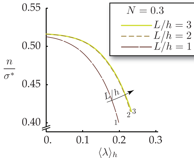
Fig. 7. Normalized load n/\sigma^* versus the additional average stretch after bifurcation in the region 0 \leq X \leq h , \langle \lambda \rangle_h \equiv x(h)/h - \lambda_c . The block material is elastic-plastic with N=0.3 and \sigma^*/E = 0.003 . As seen above, this relation is essentially independent of the initial aspect ratio if L/h \geq 2 , and these curves are virtually unchanged when \sigma^*/E is increased from 10^{-3} to 10^{-2} .
