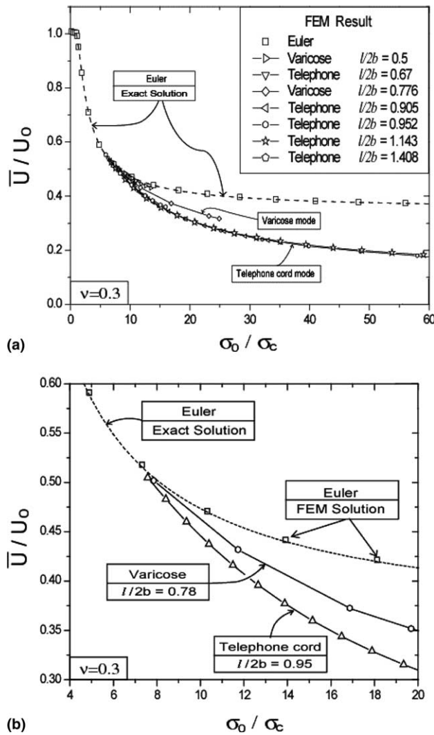
Fig. 7. Ratio of the average energy per unit area in the buckled state to that in the unbuckled state, \bar{U}/U_0 , as a function of \sigma_0/\sigma_C for \nu = 0.3 for three modes: the Euler mode, the symmetric varicose mode, and the asymmetric telephone cord mode. In (a), results for various wavelengths, l/2b , are shown for the two undulating modes. In (b), results are given for the wavelength associated with bifurcation. Only the Euler mode exists for \sigma_0/\sigma_C < 6.5 . Only the telephone cord mode is stable for \sigma_0/\sigma_C > 6.5 . The exact result for the Euler mode is given by (8).
