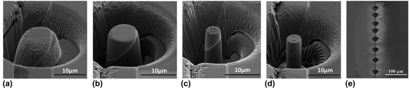
FIG. 3. Fabrication of cylindrical micro-pillar with scripted \text{Ga}^+ FIB milling: the SE images (a), (b), (c), and (d) show successive stages of ion milling to shape a portion of a CrN/Cu/Si specimen into a micro-pillar without significant taper, with interfaces inclined at 45^\circ to the pillar axis. The SE image shown in (e) shows one array of finished micro-pillars.
