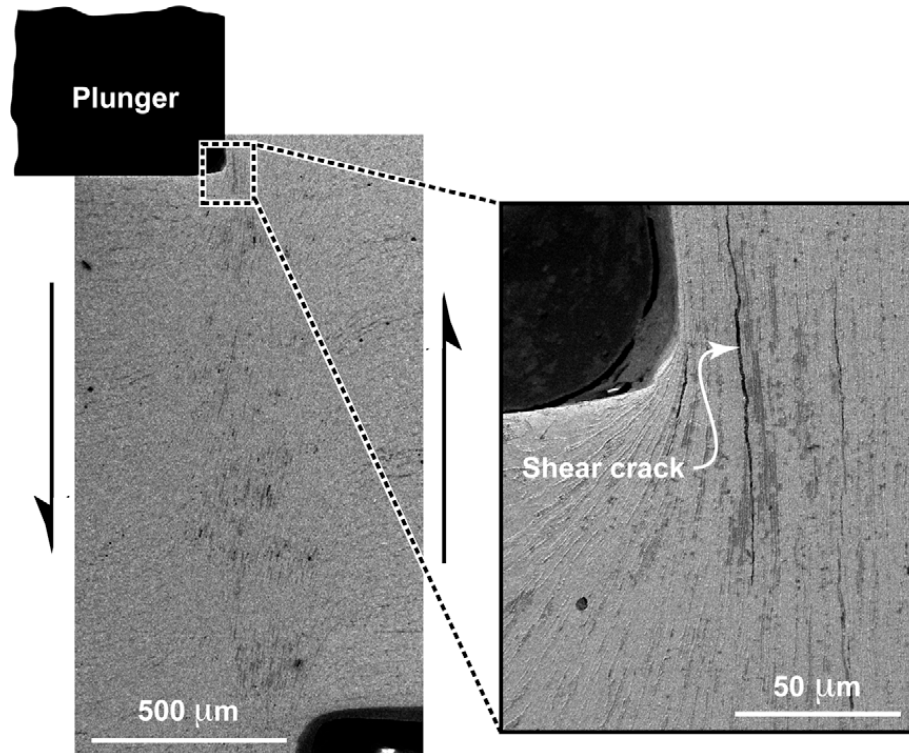
Fig. 11. Scanning electron micrographs of polished cross-sections through shear-out specimen, interrupted at displacement \delta/H = 0.5 .
