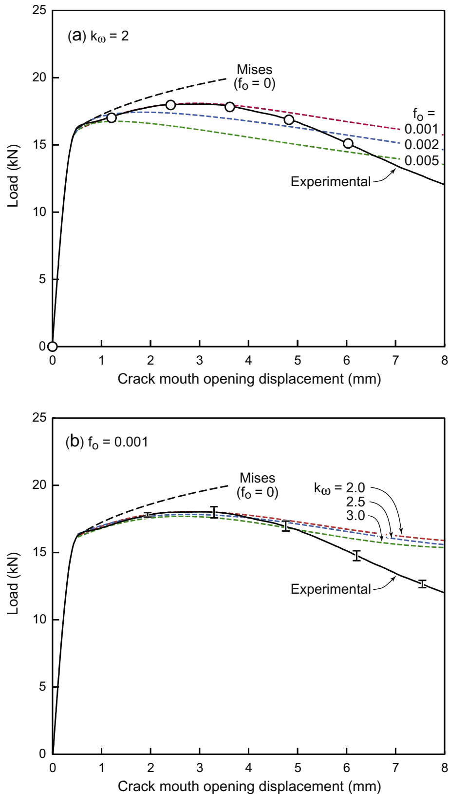
Fig. 6. Effects of (a) f_0 and (b) k_\omega on the load–displacement response of compact tension tests. Error bars represent the full range of experimental measurements from five tests. Tests were performed at a displacement rate of 1.2 mm/min. Open circles in (a) correspond to images in Fig. 7.
