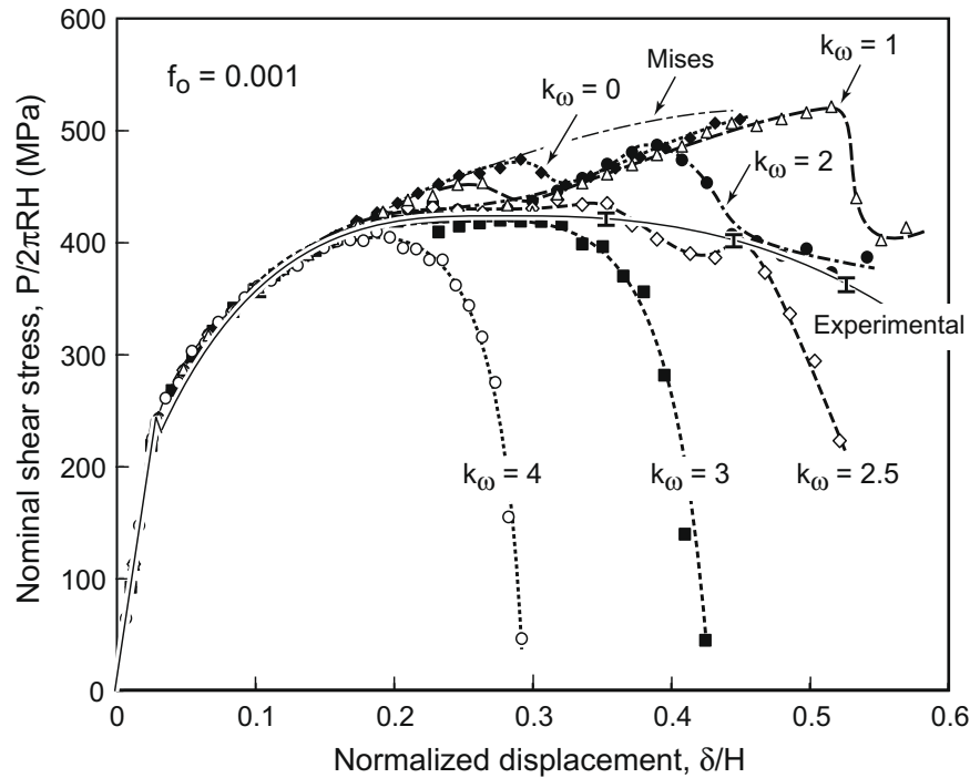
Fig. 10. Measured and computed shear-off response.
