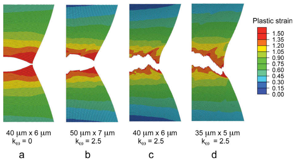
Fig. 14. Effects of initial element size and k_{\omega} on the crack trajectory in an initially unnotched round tensile bar.
