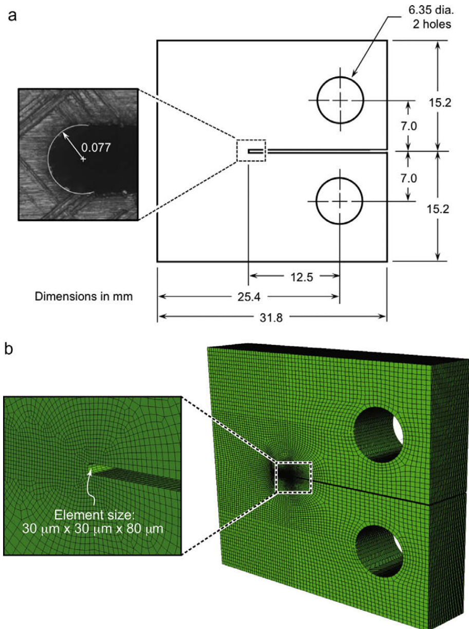
Fig. 5. (a) Compact tension test geometry employed in the experimental study and (b) corresponding finite element model. Specimen thickness is 12.5 mm. Crack mouth opening displacements were measured using a non-contacting extensometer and a pair of fiducial tapes mounted on the specimen edge, separated by a distance of 14 mm. The same definition was used in the subsequent finite element calculations.
