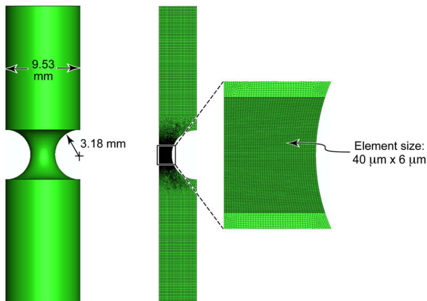
Fig. 16. Notched tensile geometry and corresponding finite element mesh.
