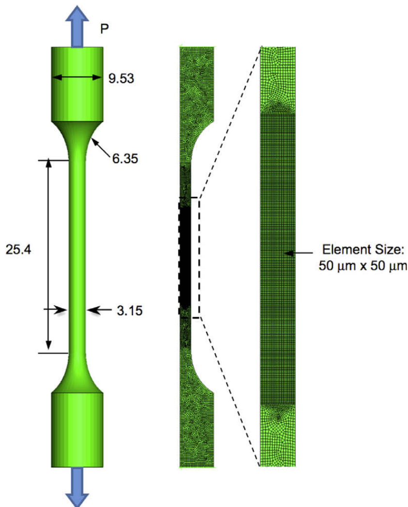
Fig. 2. Tensile specimen geometry and finite element mesh.
