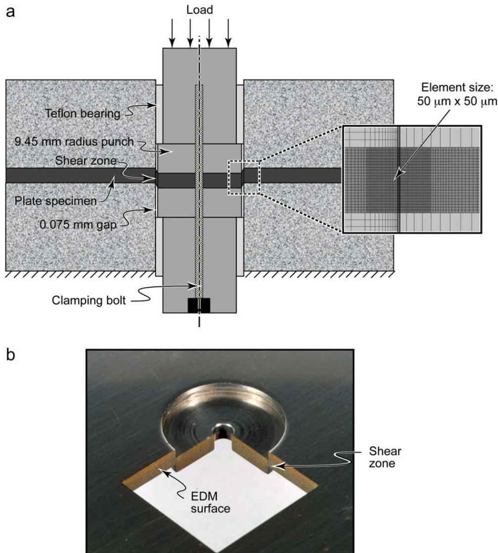
Fig. 9. (a) Shear-off test assembly and detail of finite element model in the region of intense plastic deformation. (b) Macro photograph of specimen interrupted during shear-off test and sectioned by electrodischarge machining (EDM).
