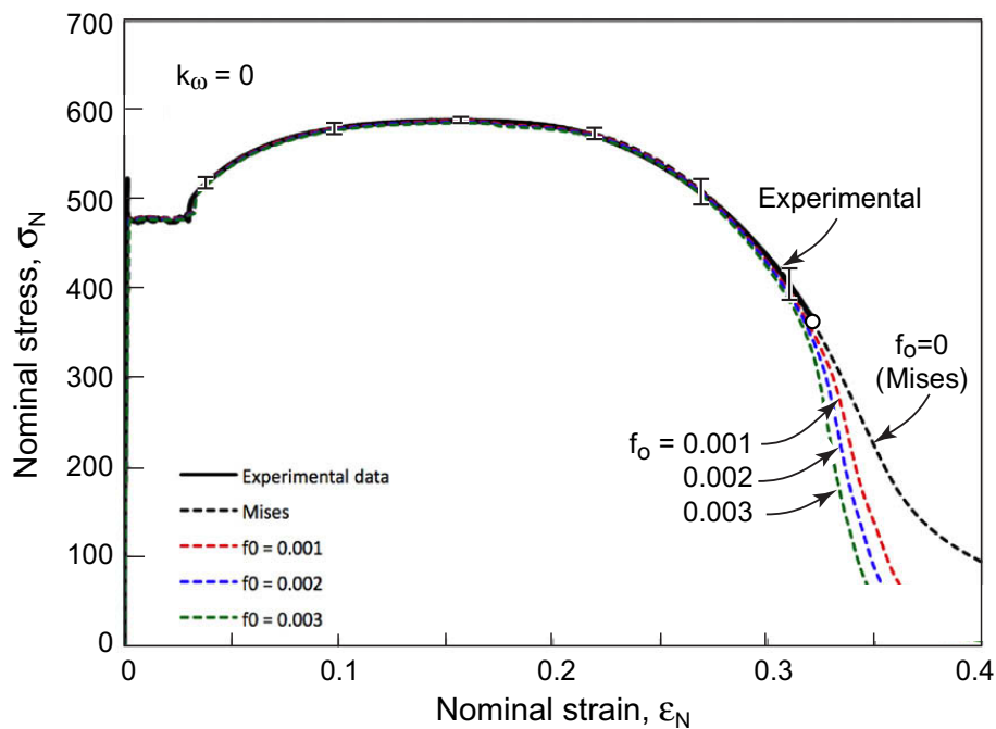
Fig. 4. Effects of initial void volume fraction f_0 on the computed nominal tensile stress–strain response. Over the pertinent range of f_0 , the computed results are indistinguishable from the experimental measurements up to the onset of fracture.
