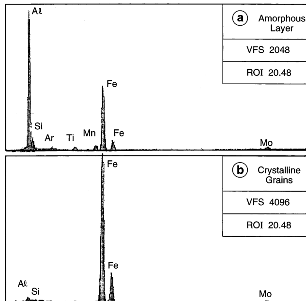
Fig. 5. (a) Energy dispersive X-ray (EDX) analysis of the amorphous oxide layer. (b) EDX analysis of one of the crystalline \alpha -Fe domains contiguous with the oxide interlayer.
