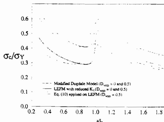
Fig. 11 Residual strength curve as given by LEFM with reduced fracture toughness ( \bar{K} = K_{IC} / (1 - D_{MSD}) ) and the modified Dugdale model for D_{MSD} = 0 and 0.5 for a stiffened sheet. The prediction of eqn (10) is also shown for D_{MSD} = 0.5 .
