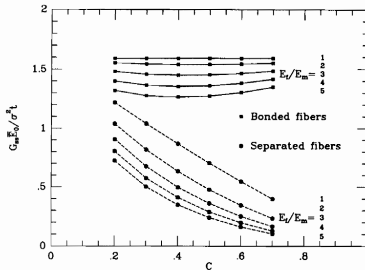
Fig. 4. The function, f(E_t/E_m, c) , providing the tunneling energy release rate in (11) for an isolated crack.
