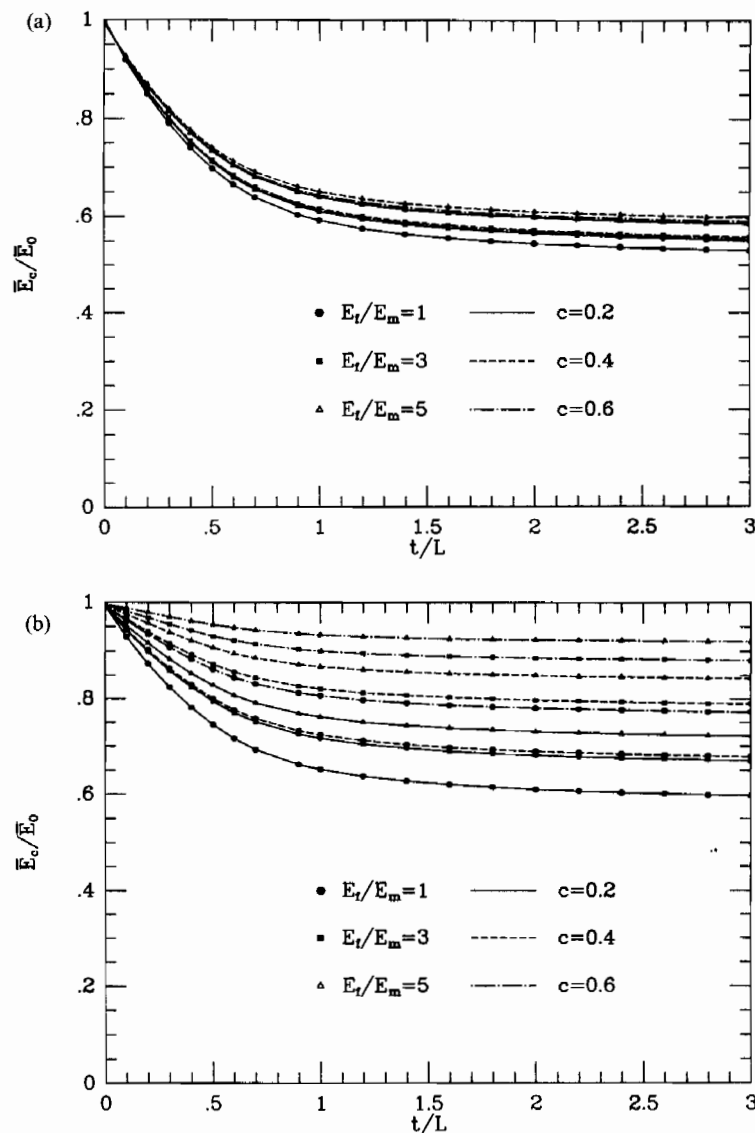
Fig. 7. The function, h(E_t/E_m, c, t/L) , providing the effective Young's modulus for the cracked laminate in (14). (a) Bonded fiber/matrix interfaces. (b) Separated fiber/matrix interfaces.
