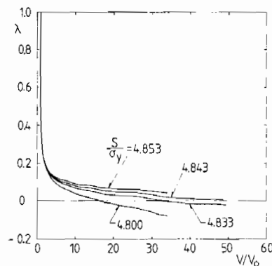
Fig. 7. — Surface load parameter \lambda vs. void volume V for spherical void, where \rho = T/S = 0.95 , \sigma_y/E = 0.003 , \nu = 0.3 and N = 0.05 . Remote strain and stress states are kept fixed.
