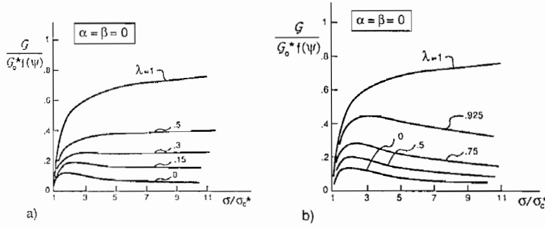
FIG. 66. Mode-adjusted crack driving force for the circular blister: a) based on (6.20); and b) based on (6.21).
