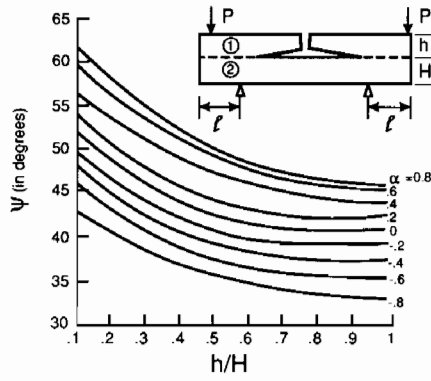
FIG. 34. The insert shows the UCSB four-point flexure of a bilayer. The mode mixity is plotted.
