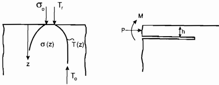
FIG. 55. A model for thermal shock spalling.
