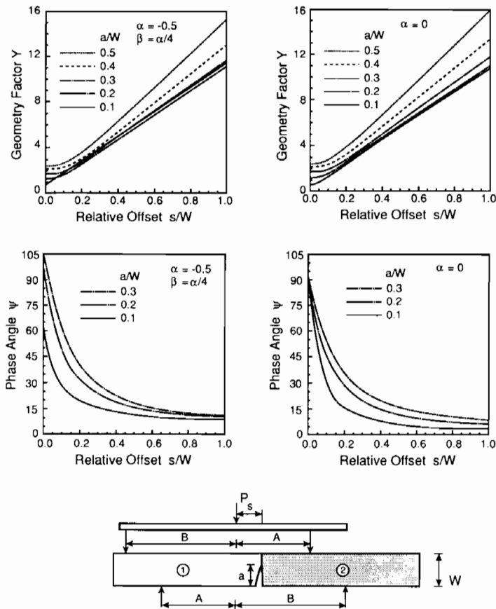
FIG. 36. Calibration of the edge-notched shear of a bimaterial bar.
