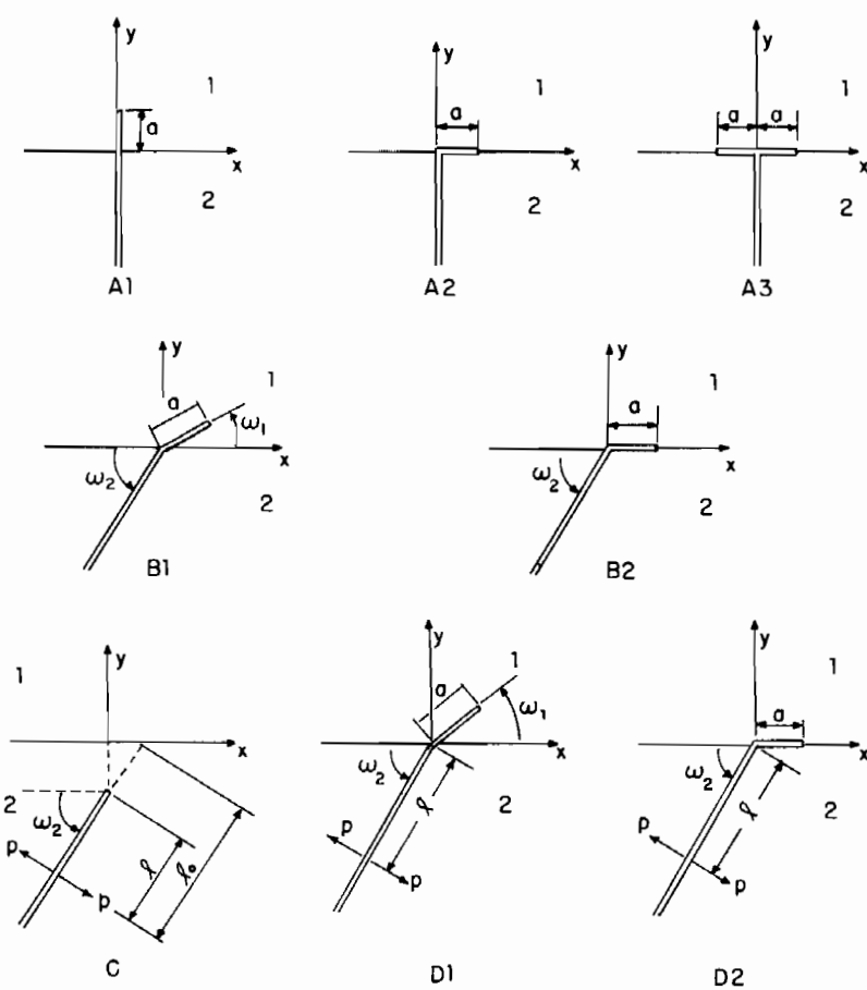
Fig. 1. Crack geometries.
