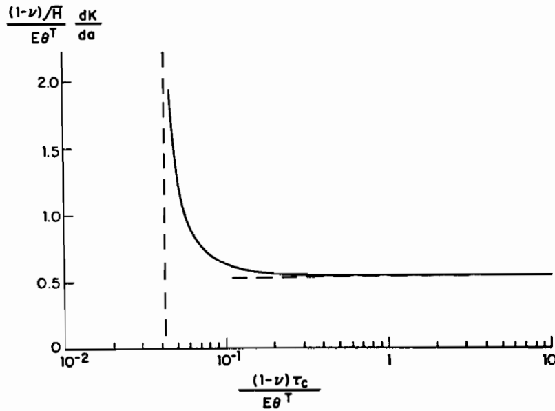
Fig. 6 Nondimensional initial slope of resistance curve for Case B where H is the transformation zone half-height at initiation of growth.
