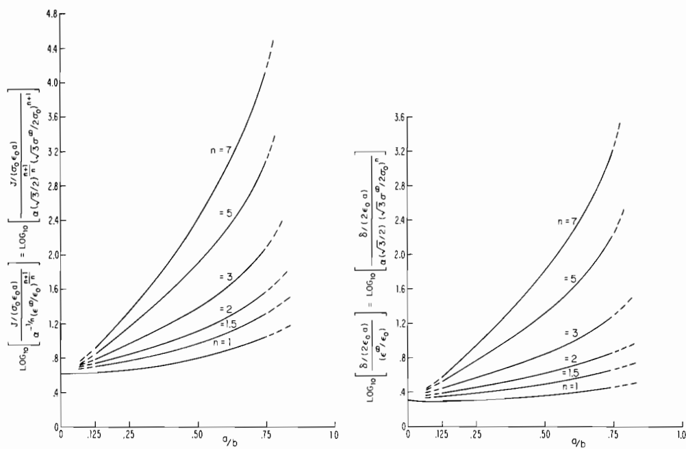
Fig. 2. Curves of J and \delta normalized with respect to \epsilon^\infty and \sigma^\infty as a function of a/b for constant values of n .
