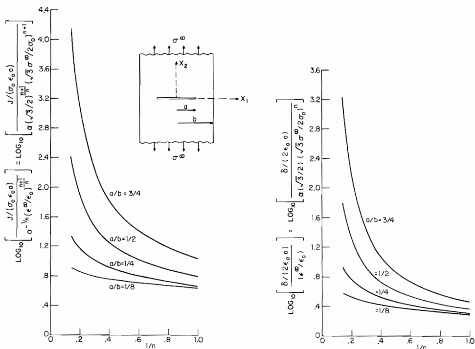
Fig. 1. Curves of J and \delta normalized with respect to \epsilon_o^\infty or \sigma_o^\infty as a function of 1/n for constant values of a/b .
