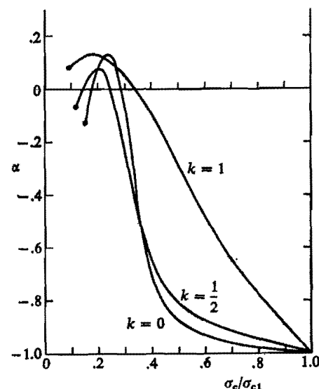
Figure 4. Postbuckling behavior as a function of buckling stress
