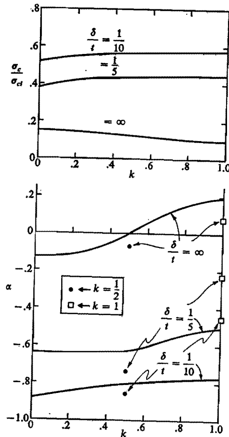
Figure 2. Variation of bifurcation stress and postbuckling parameter as a function of k for fixed values of imperfection ( v = \frac{1}{3} )
