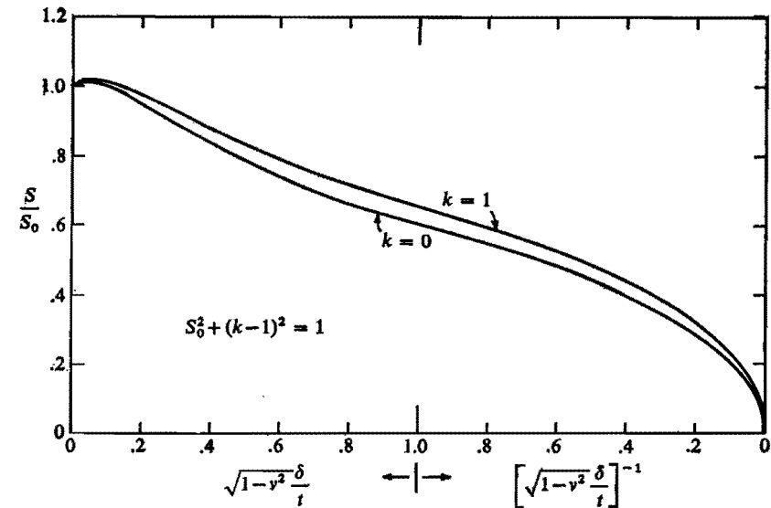
Figure 3. Critical circumferential wavelength parameter as a function of imperfection amplitude
