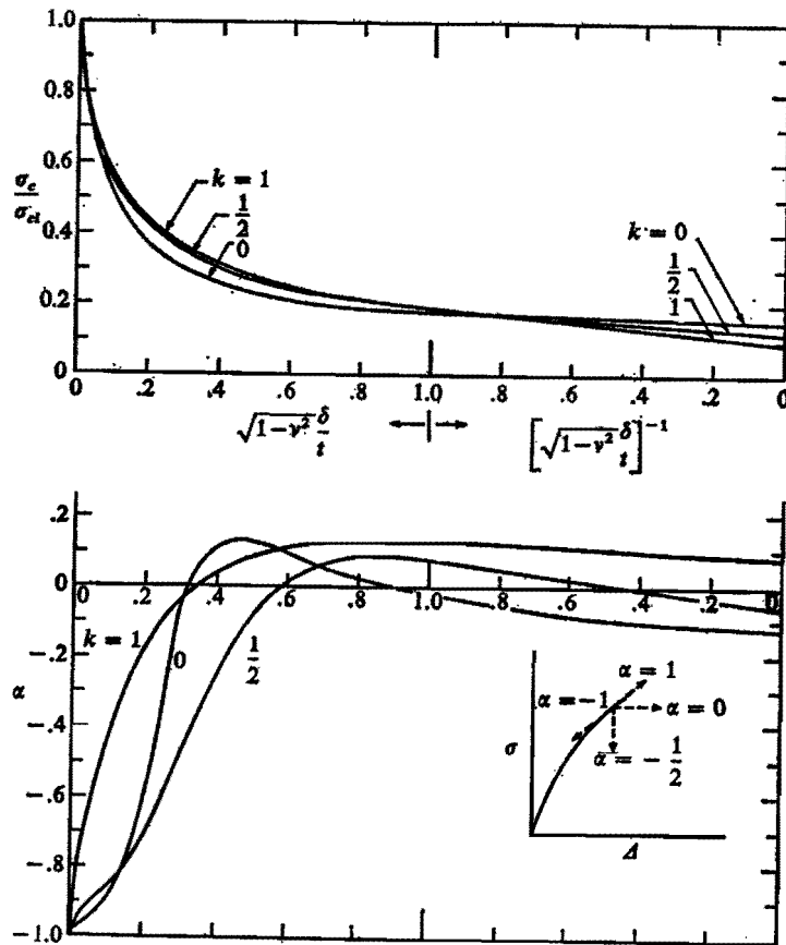
Figure 1. Buckling and postbuckling of imperfect cylindrical shells under axial compression
