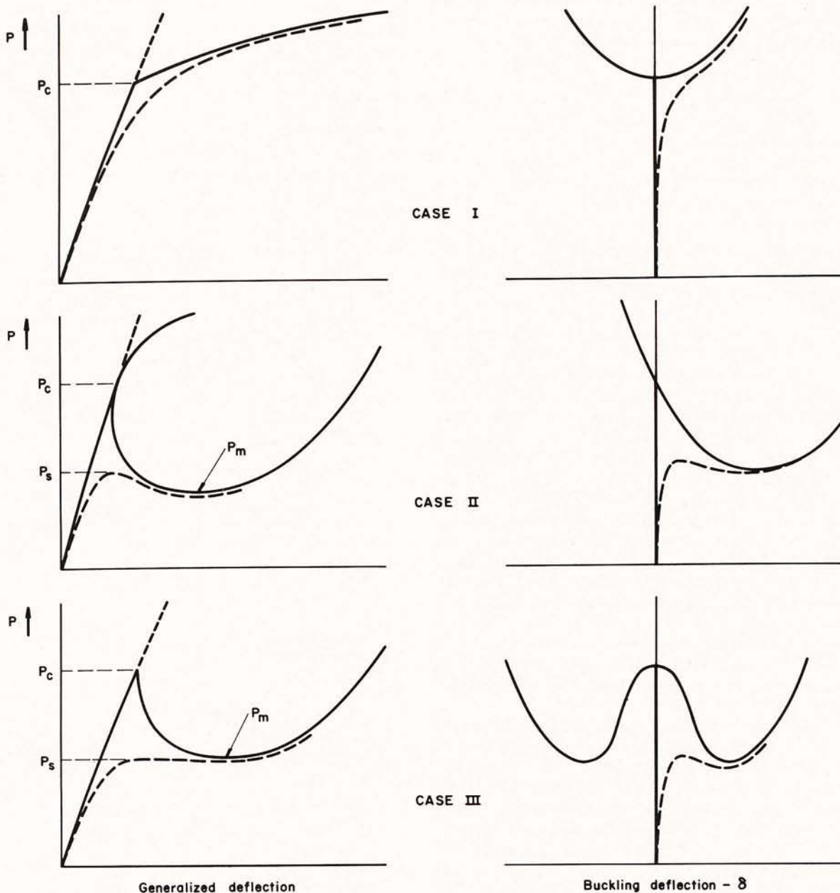
FIG. 1. LOAD-DEFLECTION CURVES FOR SINGLE MODE BIFURCATION BEHAVIOR
