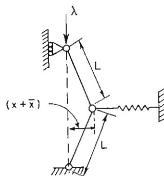
Fig. 1 Idealized column constrained by nonlinear spring.
